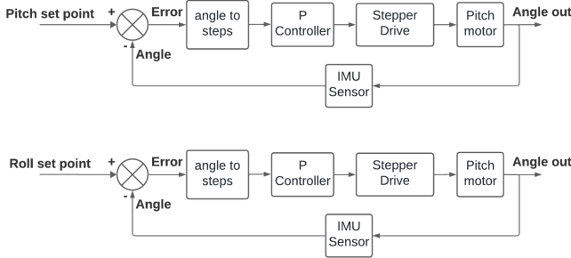
Fig. 10. Control diagram
