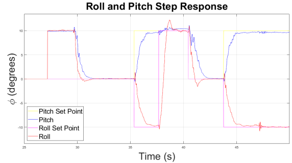
Fig. 11. Sequentially Step responses
