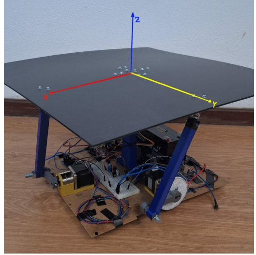
Fig. 4. Referential rotation point
