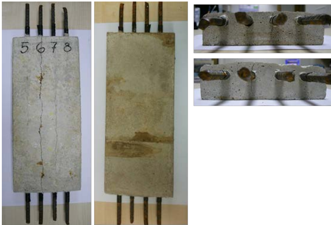
Fig. 1: short rolled bars embedded in concrete slabs.
